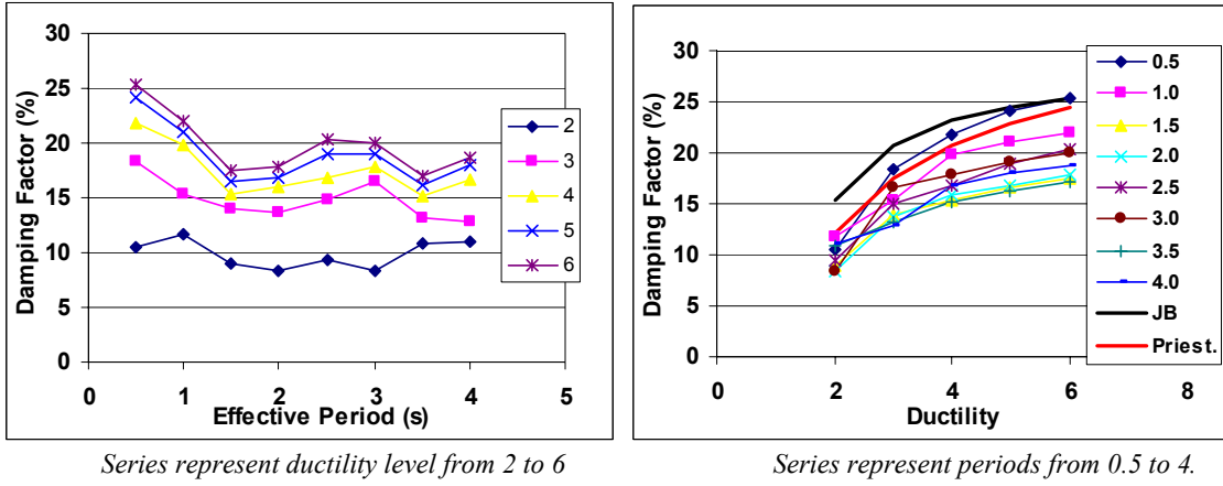
Figure 7-5 Average Equivalent Damping for Takeda model (Fat type, \alpha = 0.3 and \beta = 0.6 )
