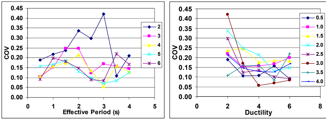
Figure 7-9 COV of EVDF for FPS Model
