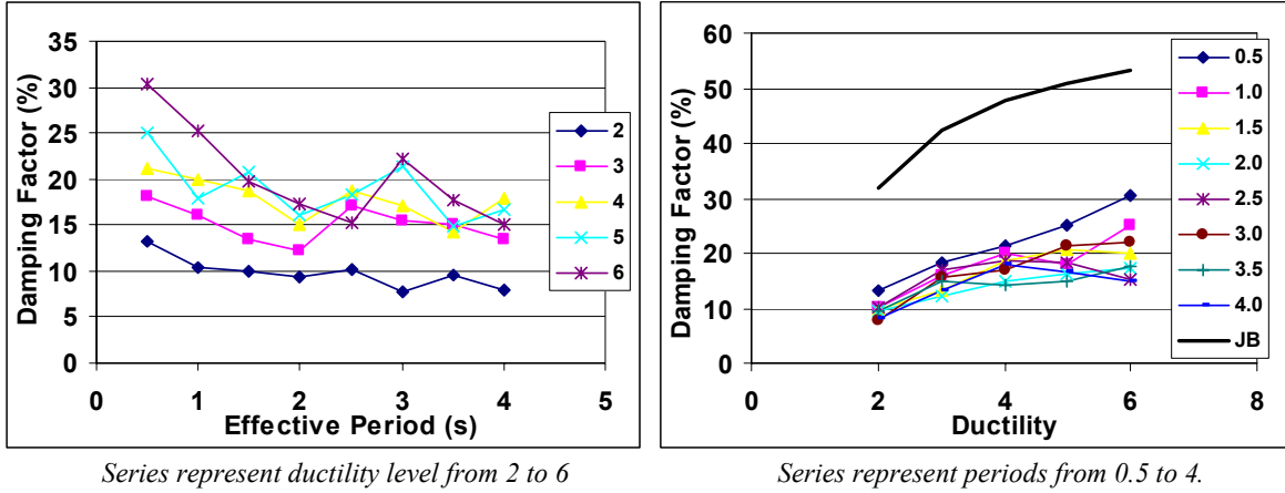
Figure 7-11 Equivalent Viscous Damping for the elastic perfectly plastic hysteretic model
