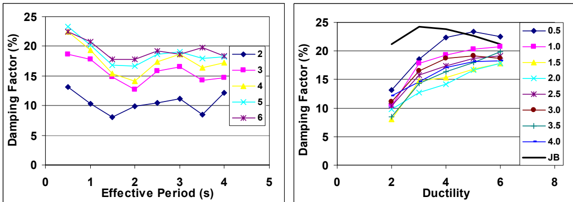
Figure 7-8 Equivalent Viscous Damping Factor for bilinear hysteretic loop ( K_1=0.2K_0 )
