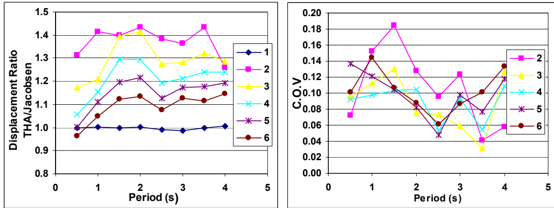
Figure 7-7 Average displacement for the bilinear hysteresis model (Jacobsen's approach)
