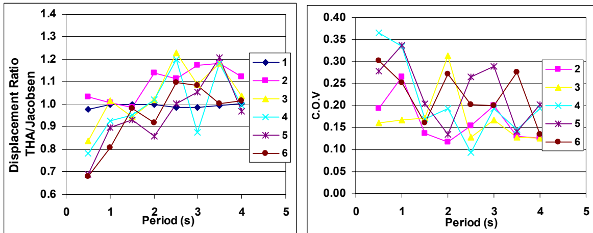
Figure 7-16 Average Displacement for ring spring model, Jacobsen approach.
