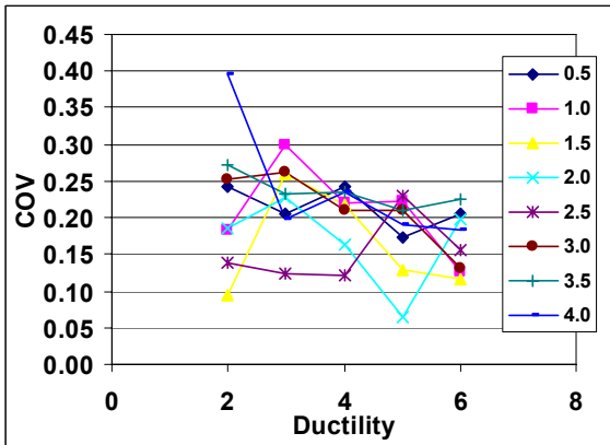
Figure 7-18 COV of the Equivalent Viscous Damping Factor for the ring spring hysteretic model.
