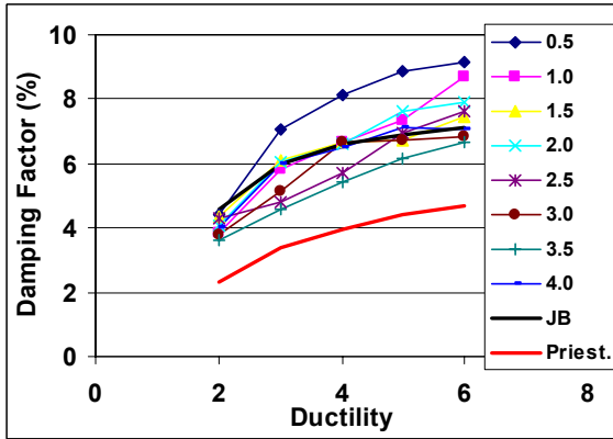
Figure 7-17 Equivalent Viscous Damping for the ring spring hysteresis model
