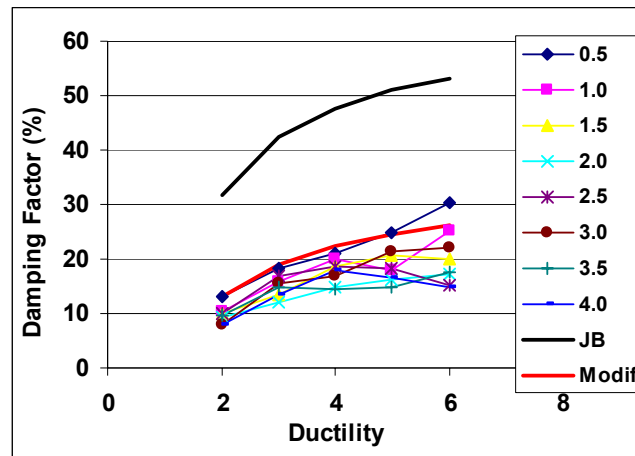
Figure 8-8 Comparison of the modified equation (red line) with Jacobsen's approach equation (black line)
