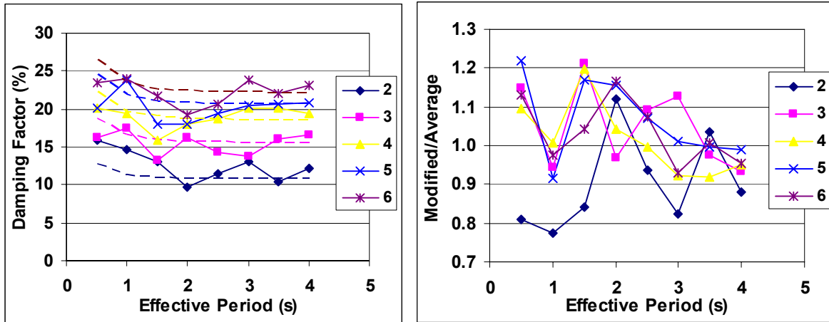
Figure 8-10 Comparison of the EVDF by the modified equation (dashed) and the average effective values (continuous) for Ramberg model.
