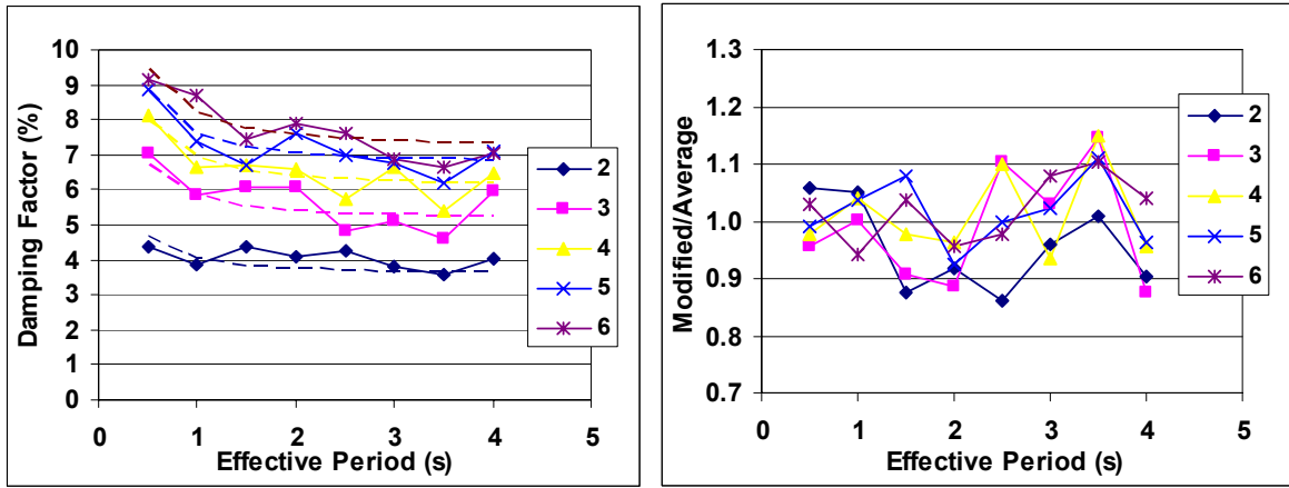
Series represent ductility level from 2 to 6 Figure 8-11 Comparison of the EVDF by the modified equation (dashed) and the average effective values (continuous) for ring spring model.
