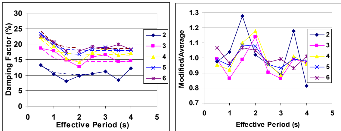
Figure 8-7 Comparison of the EVDF by the modified equation (dashed) and the average effective values (continuous).
