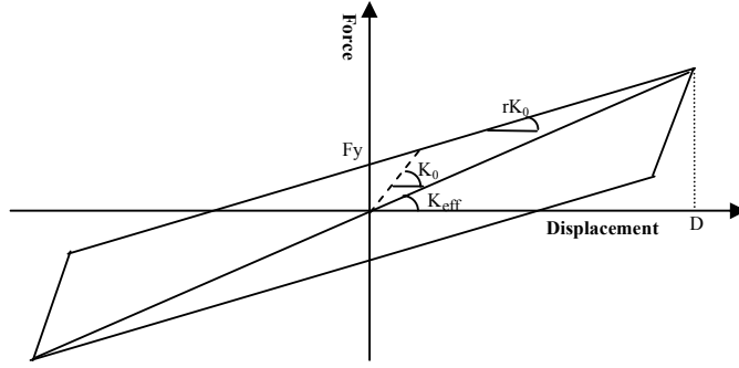
Figure 6-4 FPS hysteretic loop.
