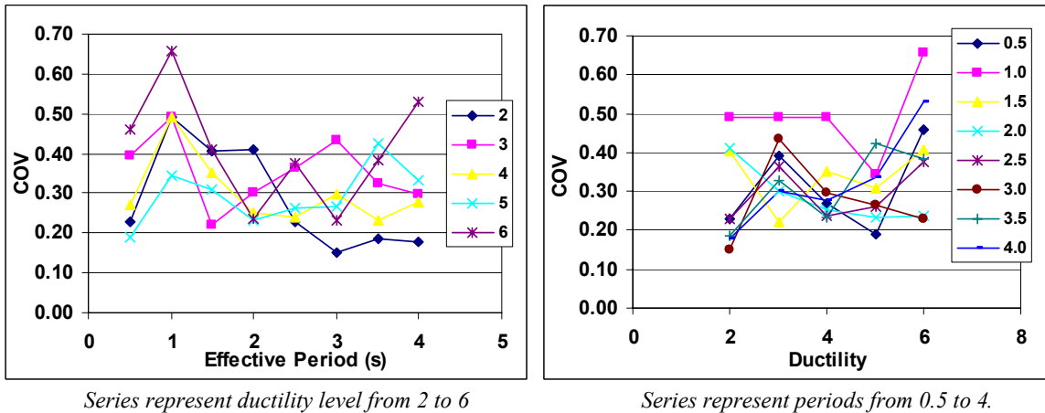
Figure 7-12 COV of the Equivalent Viscous Damping Factor for the elastic perfectly plastic hysteretic model.
