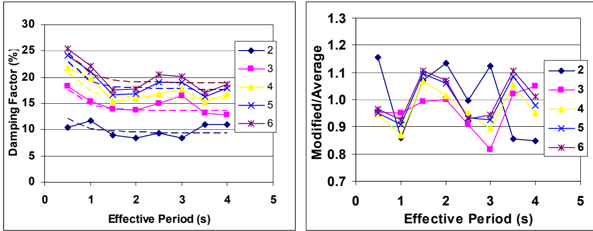
Figure 8-5 comparison of the EVDF by the modified equation (dashed) and the average effective values (continuous). (fat type)
