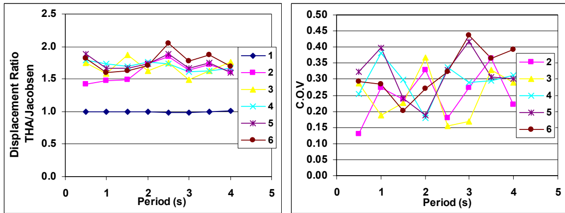
Figure 7-13 Average Displacement for Ramberg Osgood hysteretic model ( \gamma \neq 7 ), Jacobsen approach.
