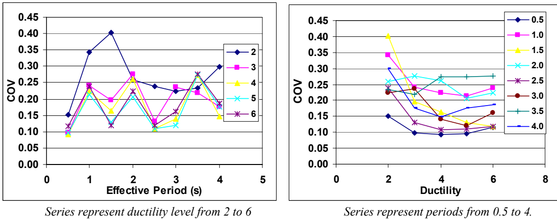
Figure 7-6 COV of EVDF for Takeda Model (Fat type, \alpha = 0.3 and \beta = 0.6 ).
