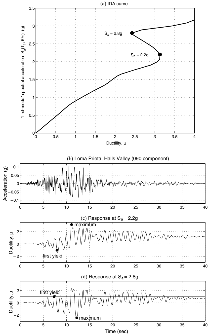
Figure 4. Ductility response of a T=1 s, elasto-plastic oscillator at multiple levels of shaking. Earlier yielding in the stronger ground motion leads to a lower absolute peak response.
