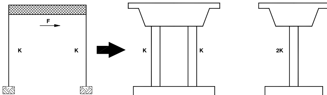
Fig. 2.1. SDOF model
