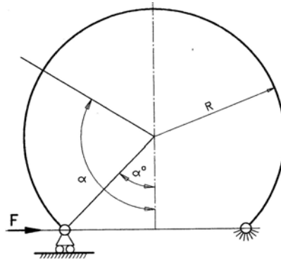
Fig. 3.14. C-shaped device static scheme
