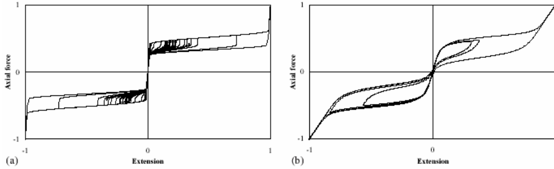
Fig. 5.9. Constitutive models for SMA finite elements: (a) Liang-Rogers and (b) Ivshin-Pence
