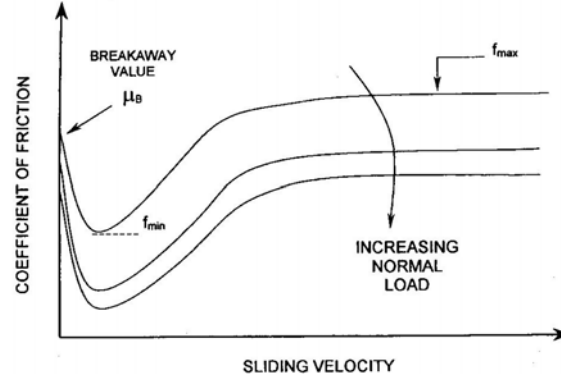
Fig. 2.10. Friction coefficient of PTFE-Polished Stainless Steel Interface at varying velocity and normal load
