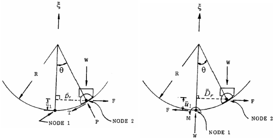
Fig. 8.11. Forces acting in F - W plane and local bending moment effect for base isolator
