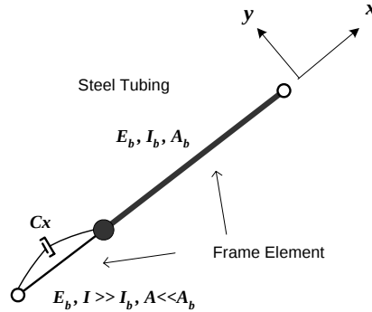
Fig. 4.8. Modeling of viscous damper and cross braces
