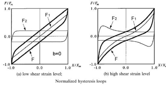
Fig. 7.15. Normalized hysteresis loops, at low and high shear strain levels respectively (Kikuchi and Aiken, 1997)
