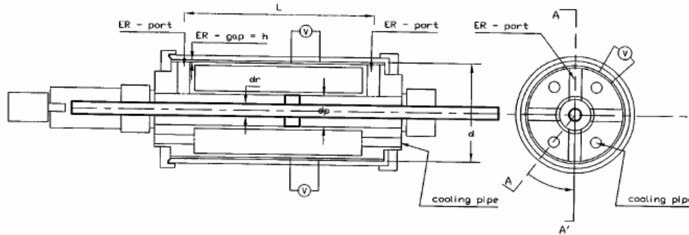
Fig. 6.12. Schematic of the new ER-damper, able to operate under high design velocities, adequate for seismic isolation systems. Section A-A is projected in line A-A
