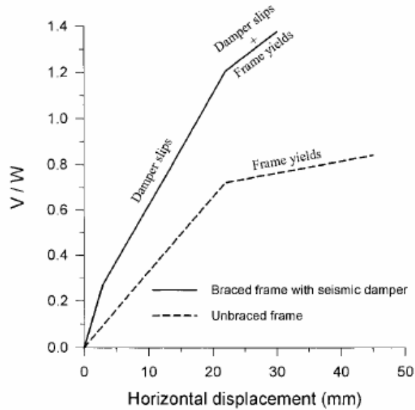
Fig. 5.15. Pushover analysis of unbraced frame and braced frame with seismic damper
