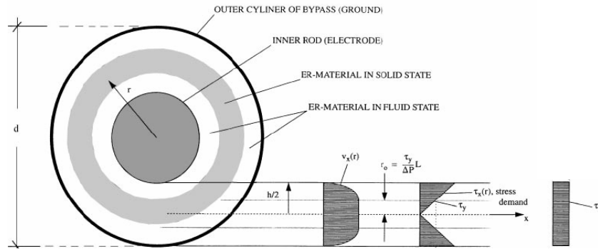
Fig. 6.10. Stress and velocity profiles of the yielding ER-fluid across the annular duct
