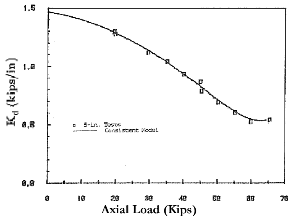
Fig. 7.19. Dynamic shear stiffness of a LRB varying the axial load (EERC)
