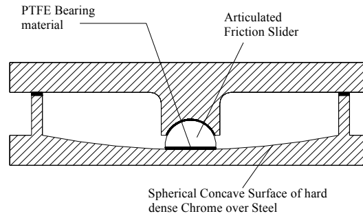
Fig. 2.22. Radial section of the FPS device
