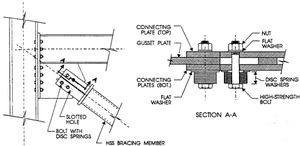
Fig. 3.4. Slotted Bolted Connection Assemblage (Tremblay and Stierner, 1993)
