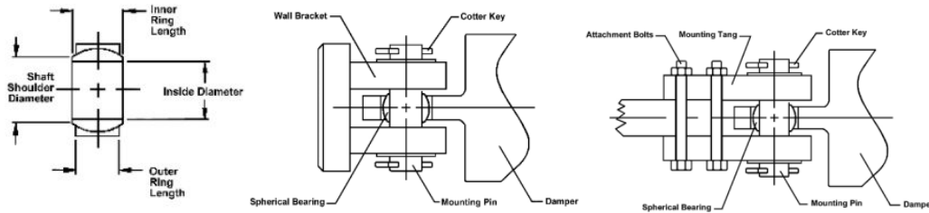
Fig. 4.11. Spherical bearing (left) and schematic of a completed attachment (center and right)
