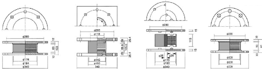
Fig. 7.17. Tested elastomeric isolation bearings, from the left: HRDB A, HRDB B, LRB, Silicon rubber bearing (Kikuchi and Aiken, 1997)
