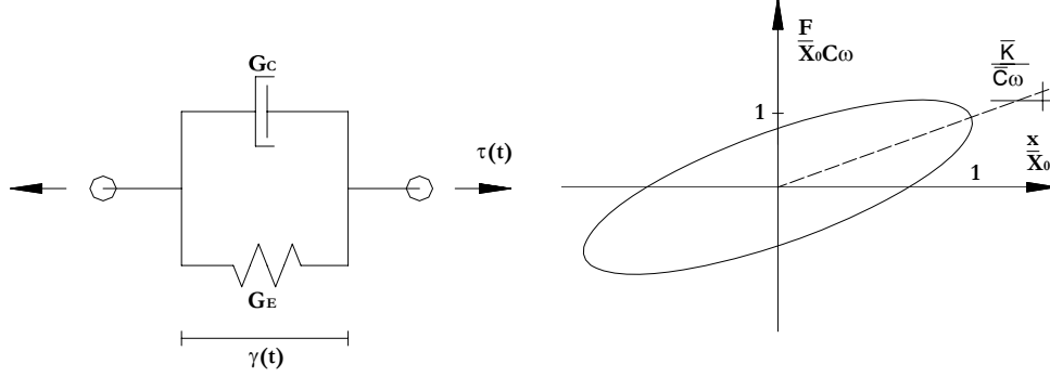
Fig. 4.17: Kelvin solid model (left) and hysteresis loop of harmonically excited viscoelastic damper (right)
