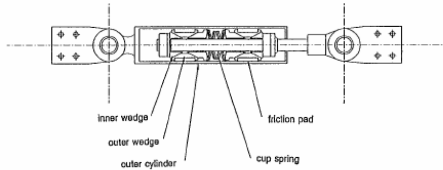
Fig. 3.8. Sectional view of the Sumitomo friction damper
