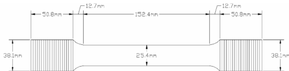
Fig. 5.1. Example of Nitinol SMA restrainer bar
