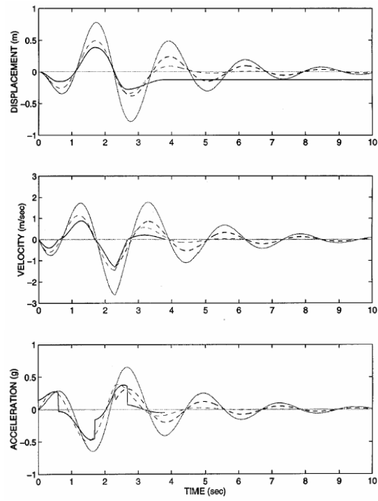
Fig. 6.14. Computed response of long-periods SDOF systems subjected to the pulse type-B, combining differently friction-type and added viscous damping.
