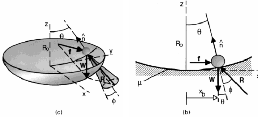
Fig. 8.4. FPS equilibrium diagrams in the 3-D (left) and 2-D (right) models
