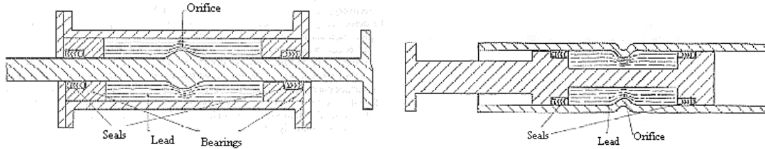
Fig. 3.21. Longitudinal section of a bulged-shaft (left) and of a constricted-tube (right) extrusion energy absorber
