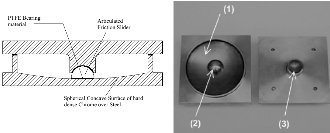
Fig. 8.1. Radial section of the FPS device (left) and components of a typical FPS (right): (1) spherical surface, (2) slider, and (3) stud
