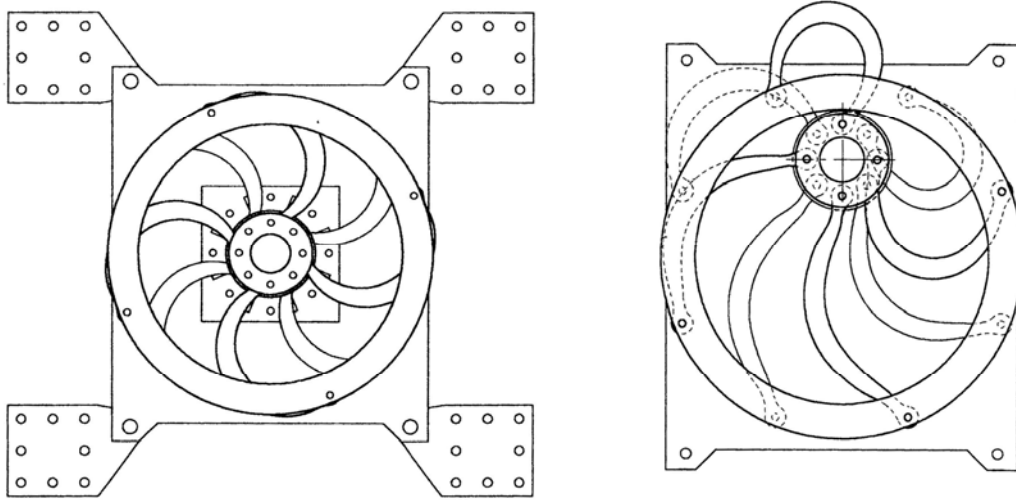
Fig. 3.15. EDU Device: device and deformed configuration
