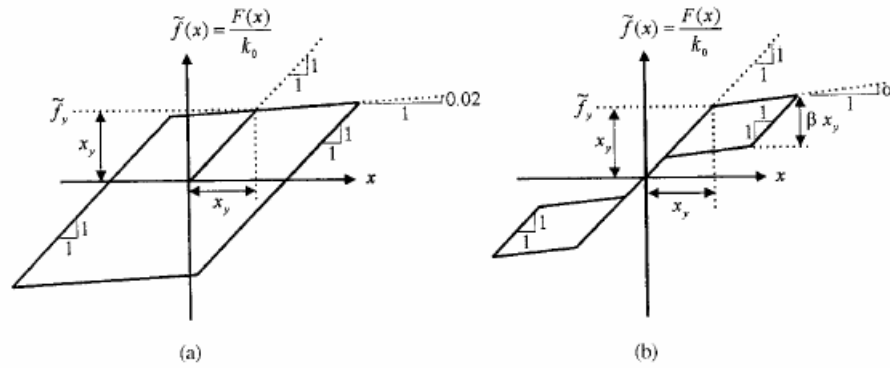
Fig. 5.19. Idealized pseudo force-displacement relationships: (a) system with welded connections; and (b) system with PTED connections
