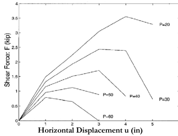
Fig. 7.20. Shear force-displacement curves as a function of the axial load
