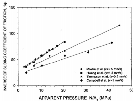
Fig. 2.9. Dependence of 1/\mu on Sliding Pressure (Constantinou et al. , 1999)
