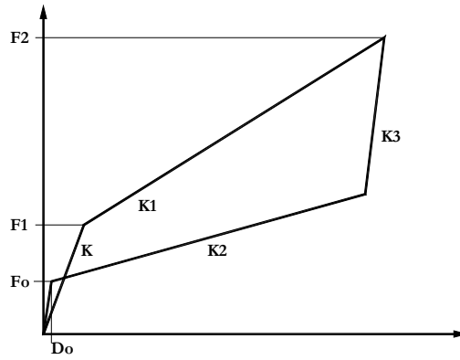
Fig. 5.21. Flag shape general hysteresis model for SC dampers
