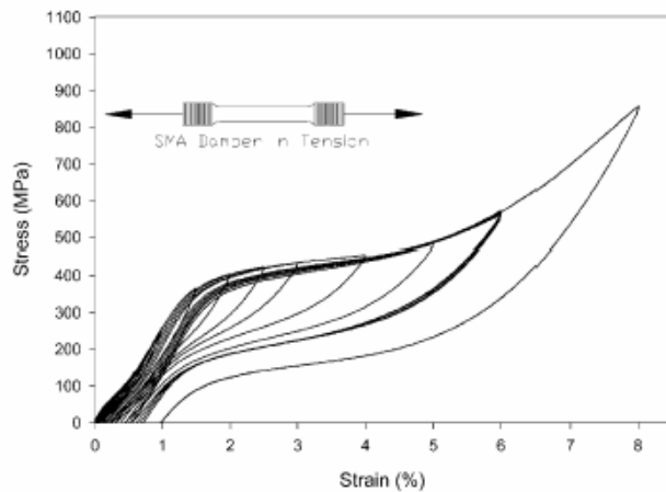
Fig. 5.5. Stress–strain curve from tension test of SMA restrainer bar (DesRoches and Delmont, 2002)
