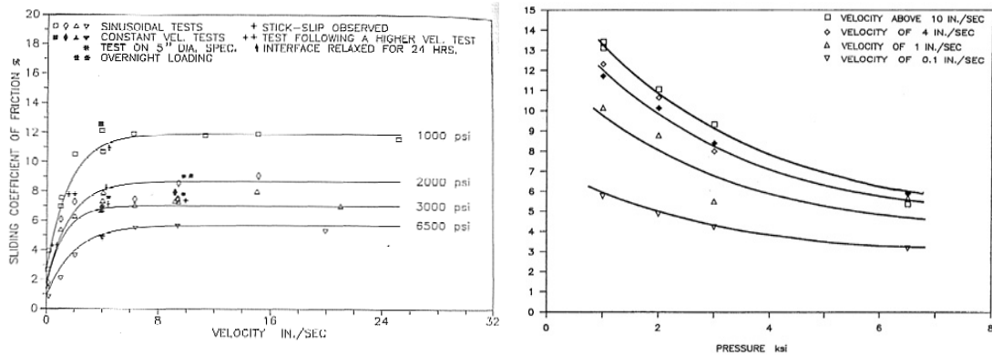
Fig. 2.12. Effect of velocity and pressure on \mu of unfilled Teflon (right), and on f_{max} of Glass-filled Teflon (Constantinou et al., 1999)
