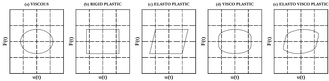
Fig. 2.5. Idealizations of energy dissipation mechanisms of practical seismic isolation systems
