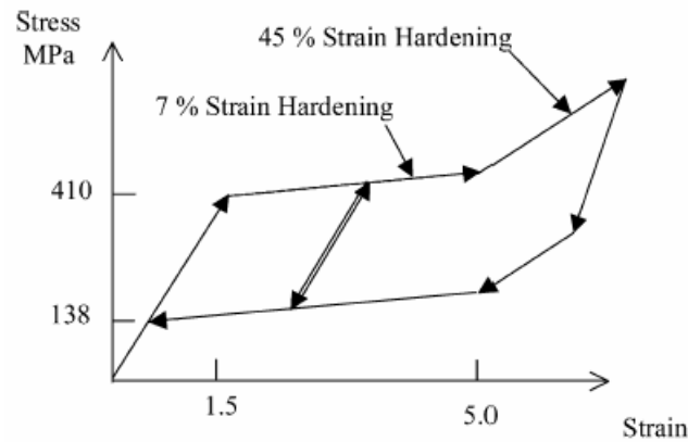
Fig. 5.8. Analytical model of SMA restrainer
