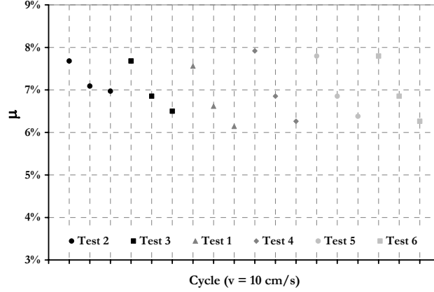
Fig. 2.16. Effect of number of cycles on the friction coefficient (on the courtesy of G. Benzoni, UCSD)
