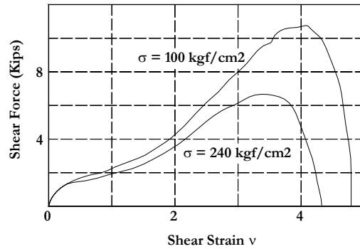
Fig. 7.18. Load-deflection relationship for the shear failure test of a HDRB (EERC)
