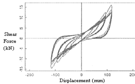
Fig. 7.11. Hysteresis loops: 100-250% shear strain sequence of a HDRB (EERC)
