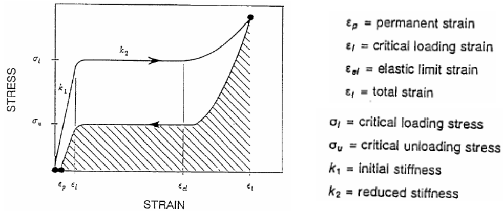
Fig. 5.3. Stress-strain relationship for superelastic shape memory alloys
