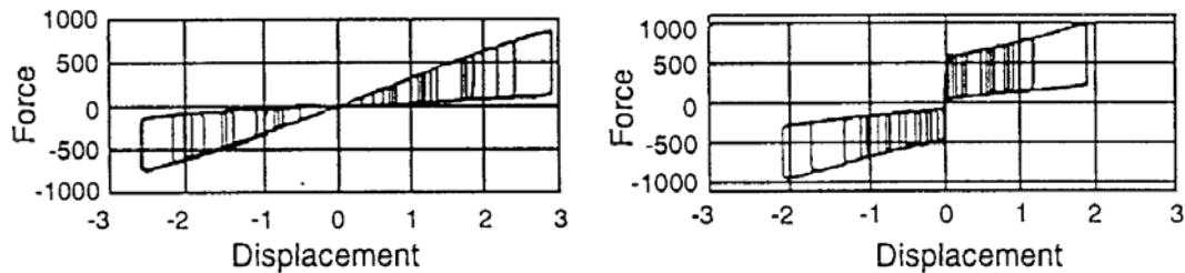
Fig. 5.11. Hysteresis loop shapes (lb-in units, Richter et al. , 1990) for EDR tested with different adjustments: left: no gap, no preload; right: no gap, some preload
