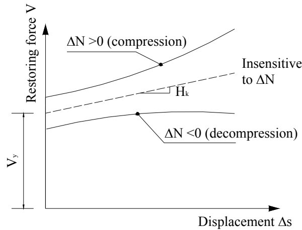
Fig. 8.9. Constitutive laws of models sensitive and insensitive models of the FPS
