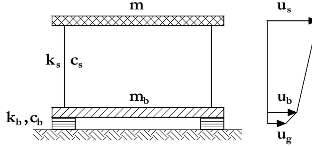
Fig. 2.3. Parameters of 2DOF isolated system
