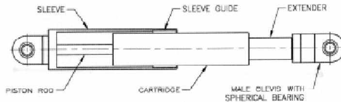
Fig. 4.1. Typical fluid viscous damper
