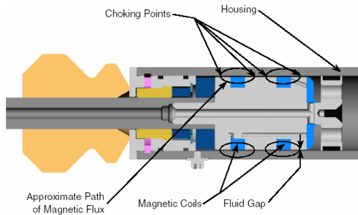
Fig. 6.3. Typical MR damper (Poynor, 2001)
