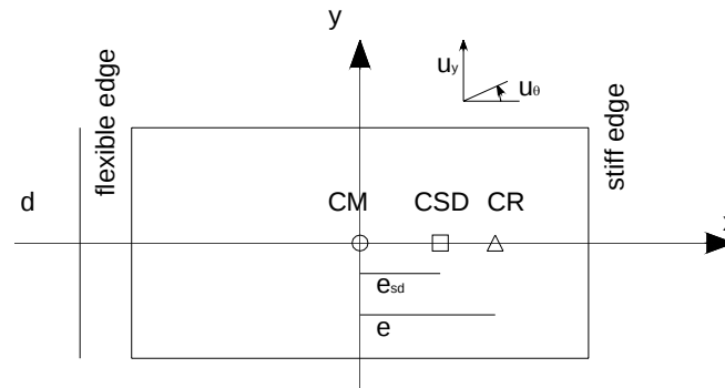
Fig. 4.13. Plan view of the one-storey system
