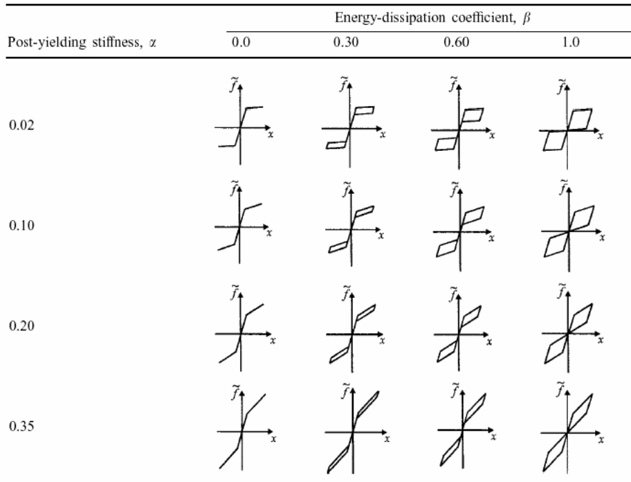
Fig. 5.20. Qualitative force-deflection relationships of flag-shaped hysteretic systems for different values of \alpha and \beta
