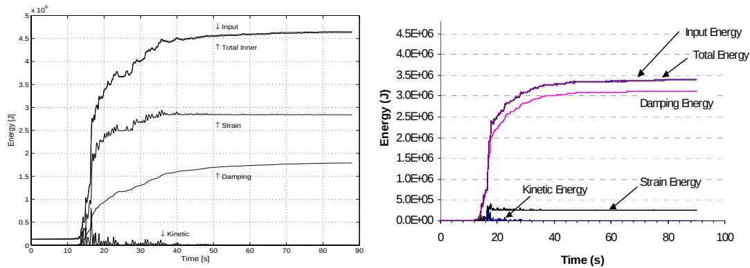
Fig. 4.9. Example of Energy balance of a structure equipped with VD, before (left) and after (right) the retrofit
