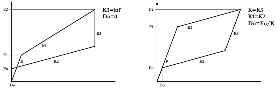
Fig. 5.23. General model in SHAPIA configuration and PTED configuration
