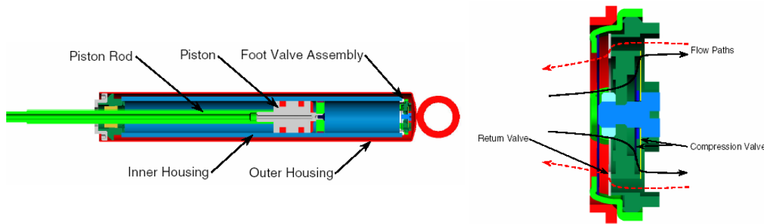
Fig. 6.5. Twin tube MR damper and detail of foot valve (Poynor, 2001)
