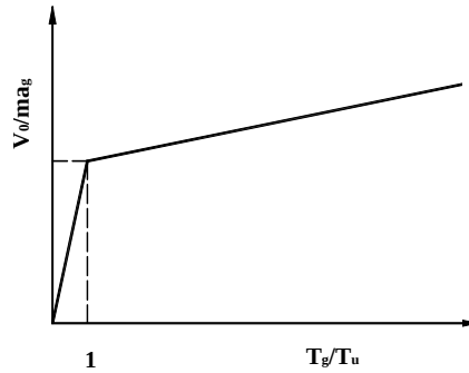
Fig. 3.23. Design-slip load spectrum
