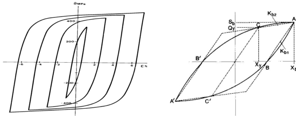
Fig. 3.10. Scaled stress-strain loops for a steel-beam damper (left) and bilinear approximation (right)
