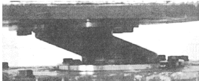
Fig. 7.12. Bearing appearance at 200% shear strain
