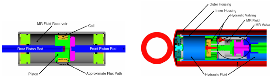
Fig. 6.6. Double-ended MR damper (left) and MR piloted hydraulic damper (right), (Poynor, 2001)
