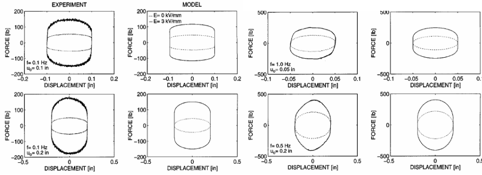
Fig. 6.11. Comparison of recorded and predicted force-displacement loops of the electrorheological damper with (solid line) and without (dashed line) electric field.
