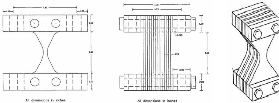
Fig. 3.17. Added Damping and Stiffness (ADAS) element
