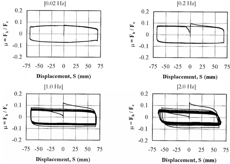
Fig. 2.6. Frictional response of unfilled Teflon-steel interface (confining pressure of 30MPa) at different load frequencies (Bondonet and Filiatrault, 1997)
