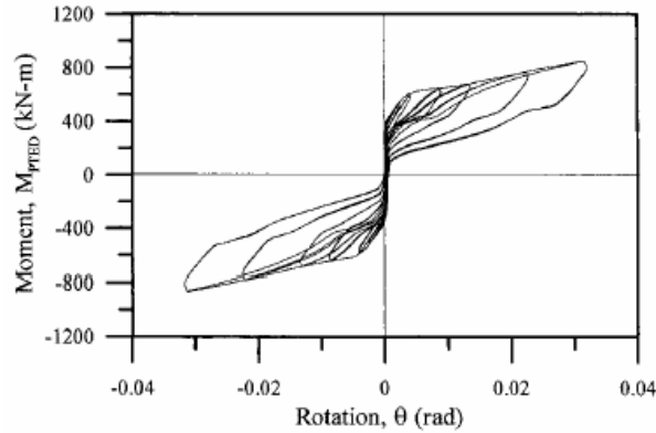
Fig. 5.17. Experimental moment-rotation curve of PTED connection
