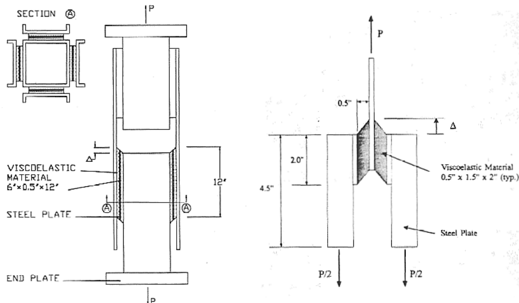
Fig. 4.15: Examples of viscoelastic dampers
