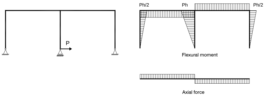
Fig. 3.12. Static Scheme of an E-shaped hysteretic damper
