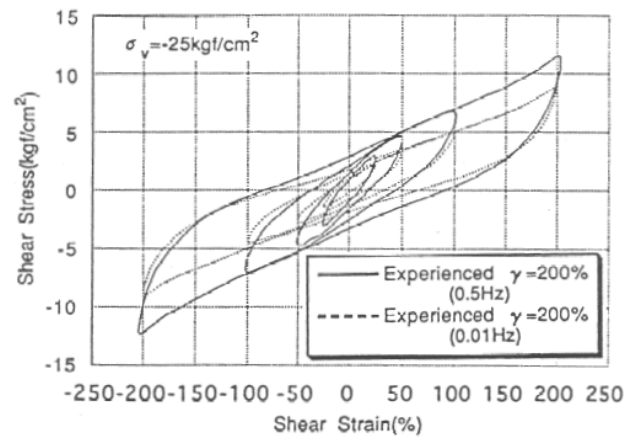
Fig. 7.6. Horizontal shear stress-strain hysteresis loop for a low shape-factor HDRB (EERC)
