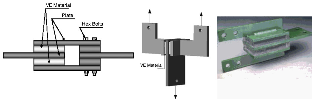
Fig. 4.14. VE damper part of a bracing member: typical scheme (front and 3D views) and picture
