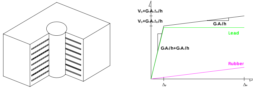
Fig. 7.7. Schematic design of a lead rubber bearing (left) and schematic bilinear constitutive law (right)
