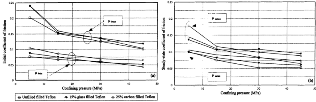
Fig. 2.8. Variations of initial (left) and steady state (right) coefficients of friction with the confining pressure (Bondonet and Filiatrault, 1997)
