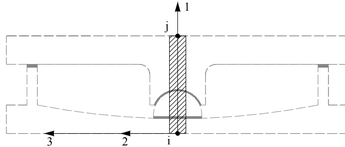
Fig. 8.12. Finite element representation of the FPS device (Calvi et al. , 2004)
