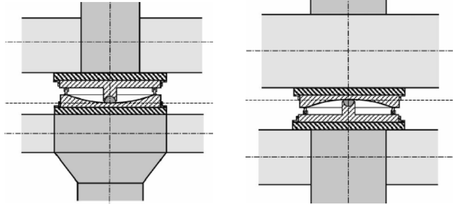
Fig. 8.3. FPS bearing in downward (left) and upward (right) position
