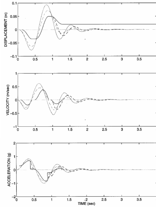
Fig. 6.13. Computed response of low-periods SDOF systems subjected to the pulse type-A, combining differently friction-type and added viscous damping
