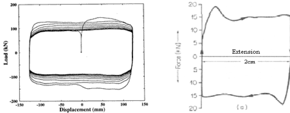
Fig. 3.22. Lead force displacement curve (left) and test results on a constricted tube absorber (right)
