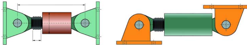
Fig. 4.12. Typical fixing detail for installation between abutment and bridge (left) and between top of pier and bridge (right)
