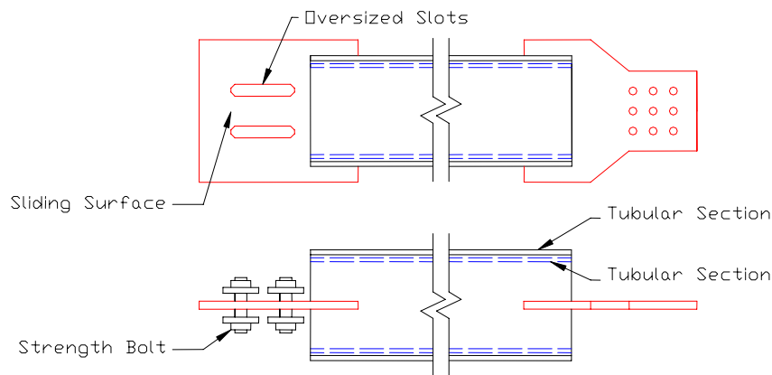
Fig. 3.5. Bracing Details
