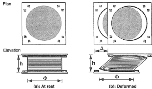
Fig. 7.3. Rubber bearing with recessed plate connection: undeformed and deformed configurations.
