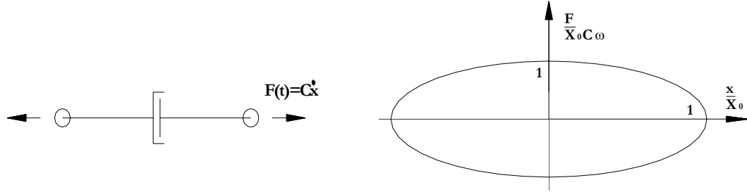
Fig. 4.3: Dashpot model (left) and cyclic response (right) of a pure viscous element
