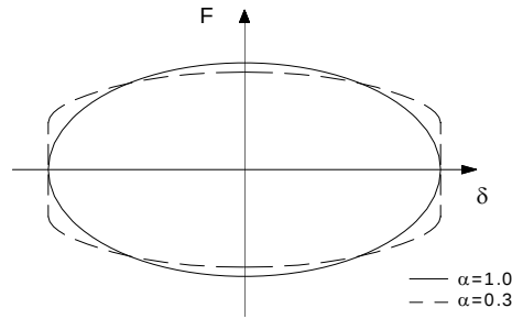
Fig. 4.4. Hysteresis loop of a viscous damper with different values of \alpha
