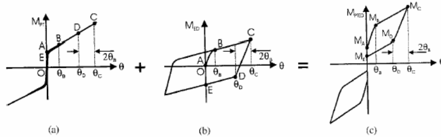
Fig. 5.18. Idealized hysteretic behaviour of the PTED connection: (a) contribution of PT Bars; (b) contribution of ED bars; and (c) moment-rotation relationship of PTED connections
