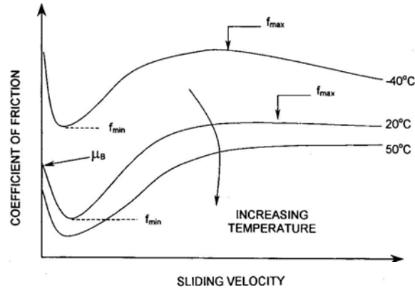
Fig. 2.15. Friction coefficient of PTFE-Polished stainless steel interface at varying velocity and temperatures
