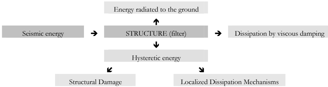
Fig. 2.2. Energy distribution at the end of an earthquake.
