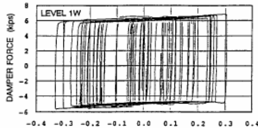
Fig. 3.9. Typical damper hysteresis loops (Aiken et al., 1993)
