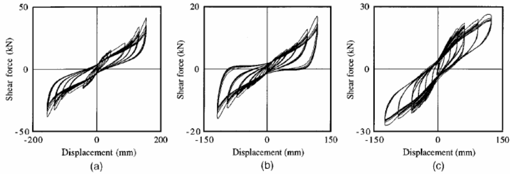
Fig. 2.21. Hysteretic loops obtained from tests of individual bearings: (a-b) high-damping; (c) lead-rubber.
