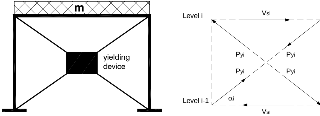
Fig. 3.3 Single Storey Friction/Metallic Damped Structure (left) and General decomposition of the braced subsystem (right)
