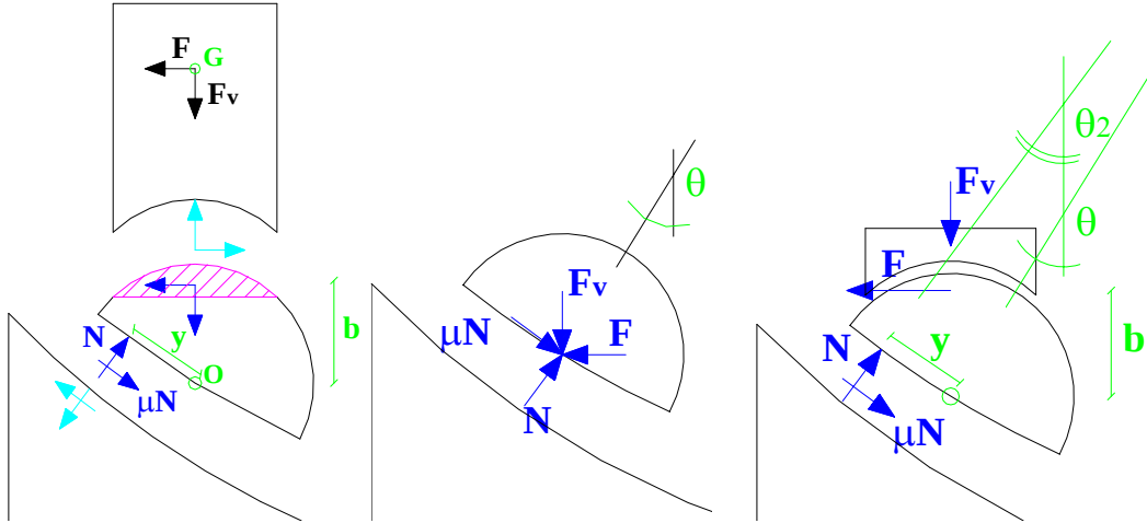
Fig. 8.8. Force transfer mechanism in the FPS: free-body diagram (left), punctual transfer mechanism approximation (center), non-punctual transfer mechanism modelisation (right)
