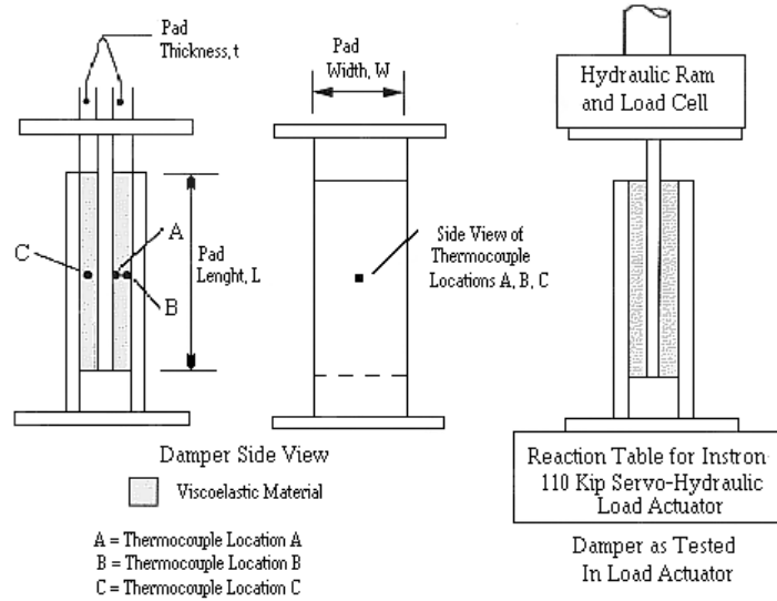
Fig. 4.16: Examples of Viscoelastic Dampers
