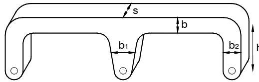
Fig. 3.11. Typical E-Shaped hysteretic damper layout
