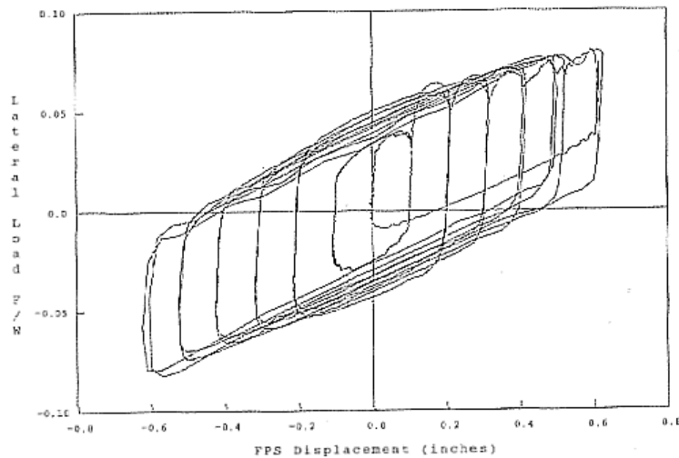
Fig. 8.2. Hysteretic response on an FPS under constant normal pressure
