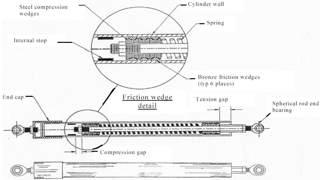
Fig. 5.10. External and internal views of the EDR (Nims et al., 1993)
