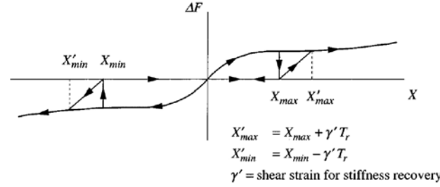
Fig. 7.16. Hysteresis rule for stiffness degradation associated with load history (Kikuchi and Aiken, 1997)
