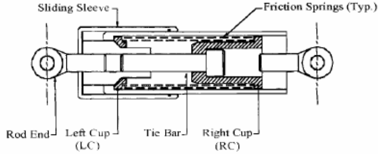
Fig. 5.13. Diagrammatic view of seismic damper
