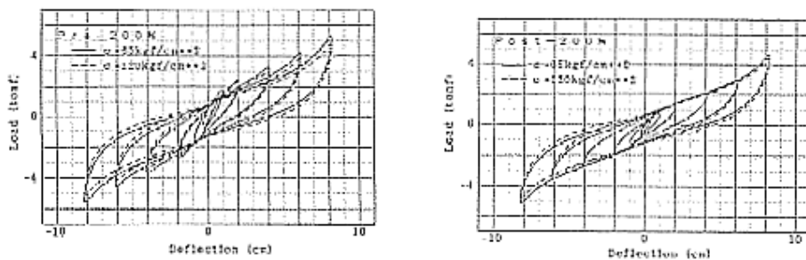
Fig. 7.13. Hysteresis loops for pre-200% (left) and post 200% (right) shear strain loading (EERC)
