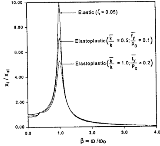
Fig. 3.2. DAF for harmonic base excitation with yielding device
