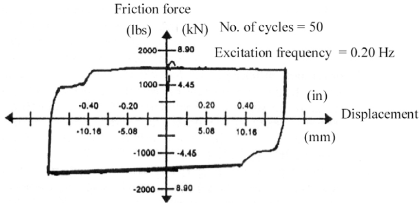
Fig. 3.7. Hysteretic loop of a Pall Friction Device
