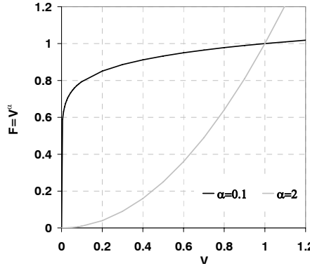
Fig. 4.2. Force-velocity type dependence for different values of the parameter \alpha
