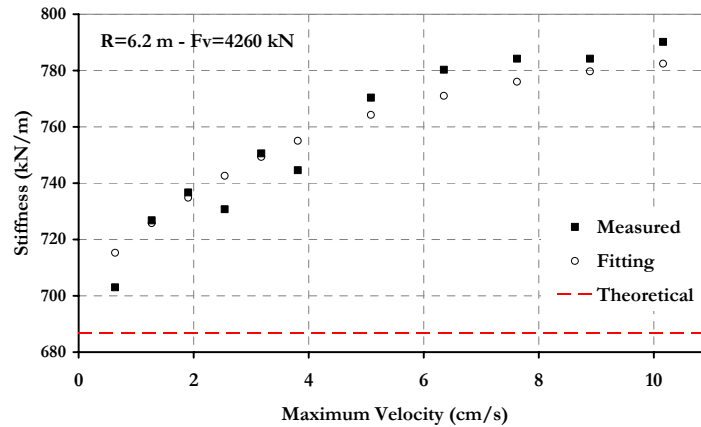
Fig. 8.6. Test results on FPS, variation of the stiffness device with the sliding velocity (small velocities range)
