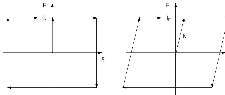
Fig. 3.1. Friction/Metallic Dampers hysteretic loops ( f_y is the slip/ yield load for friction/yielding dampers)
