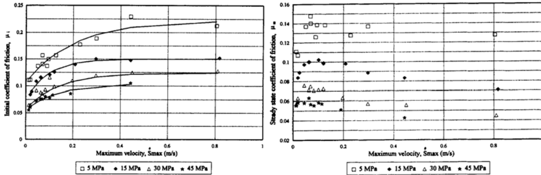
Fig. 2.7. Variations of initial (left) and steady state (right) coefficients of friction with absolute maximum velocity (Bondonet and Filiatrault, 1997)
