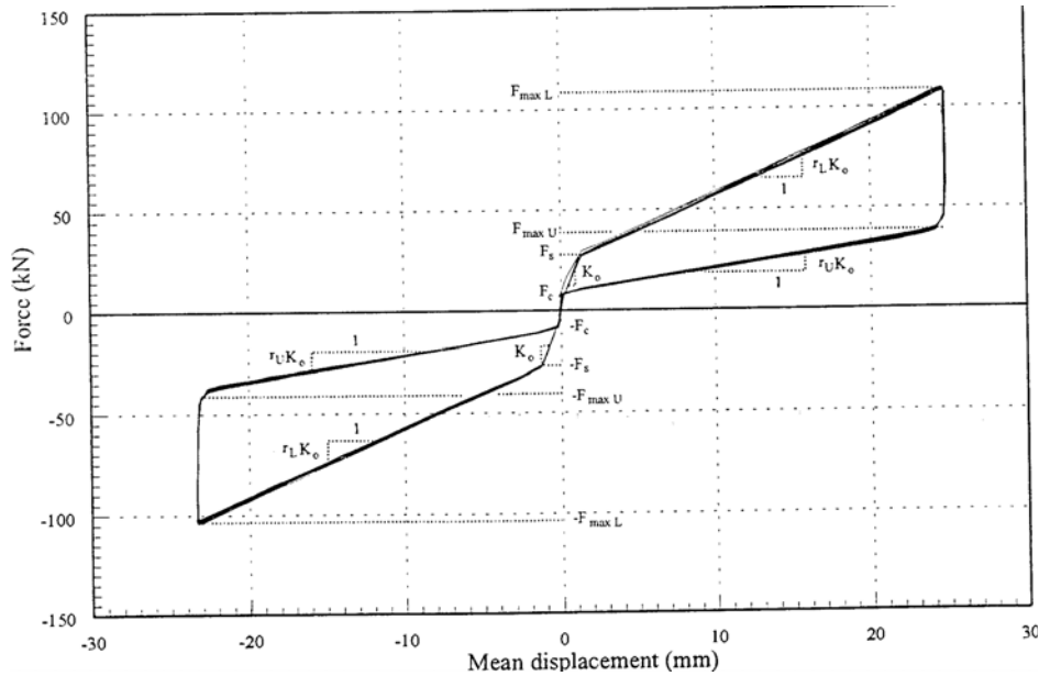
Fig. 5.14. Experimental force-displacement hysteresis loops of seismic damper
