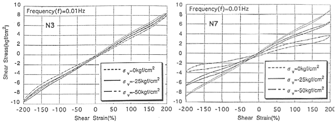
Fig. 7.4. Horizontal shear stress-strain hysteresis loop of low-shape factor natural rubber bearings (EERC), 31.5 mm (left) and 73.5 mm (right) high
