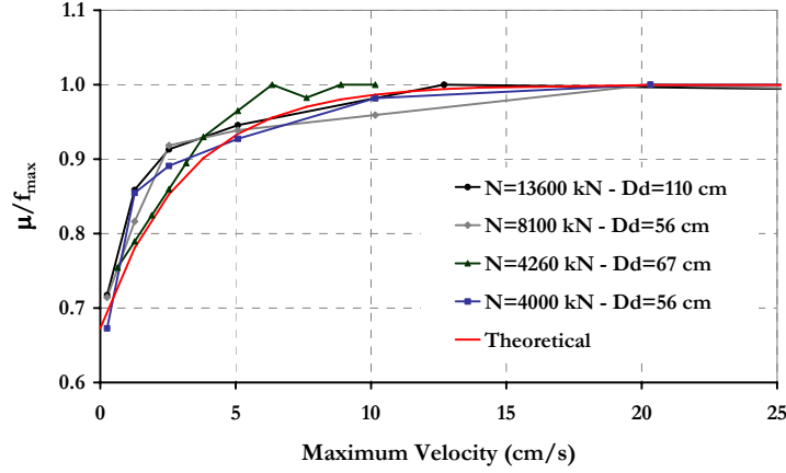
Fig. 2.14. Normalised friction coefficient-velocity dependence: theoretical vs experimental for different bearing pressures and design displacements: zoom in the small velocities range (on the courtesy of G. Benzoni)
