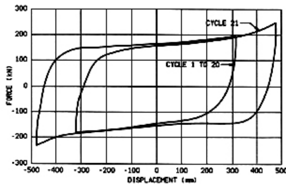
Fig. 3.16. Load deflection plot of the EDU device (Marioni, 1996)
