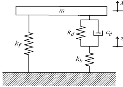
Fig. 4.19. SDOF system with an elastically supported visco-elastic damper
