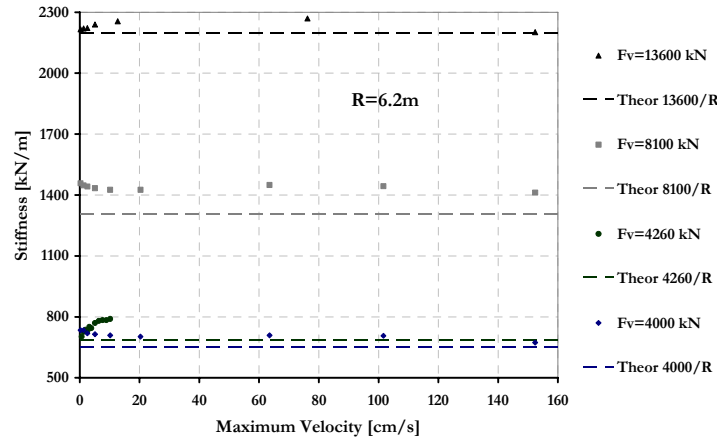
Fig. 8.5. Test results on FPS, variation of the stiffness device with the sliding velocity
