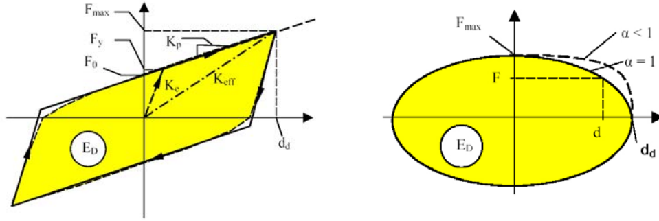
Fig. 2.18 General hysteretic behaviour (left) and viscous behaviour (right)
