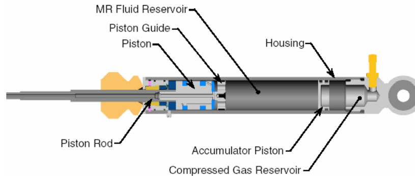
Fig. 6.4. Monotube MR damper section view (Poynor, 2001)
