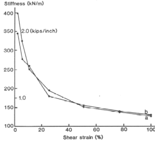
Fig. 7.14. Variation of the shear stiffness with shear strain for bearing with different shim thickness ( a=0.3 mm, b=1 mm; EERC)
