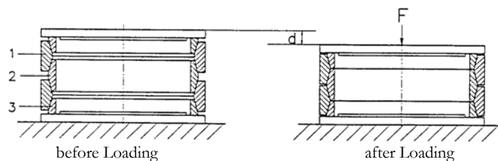
Fig. 5.12. Friction spring details. 1—outer ring; 2—inner ring; 3—inner half ring
