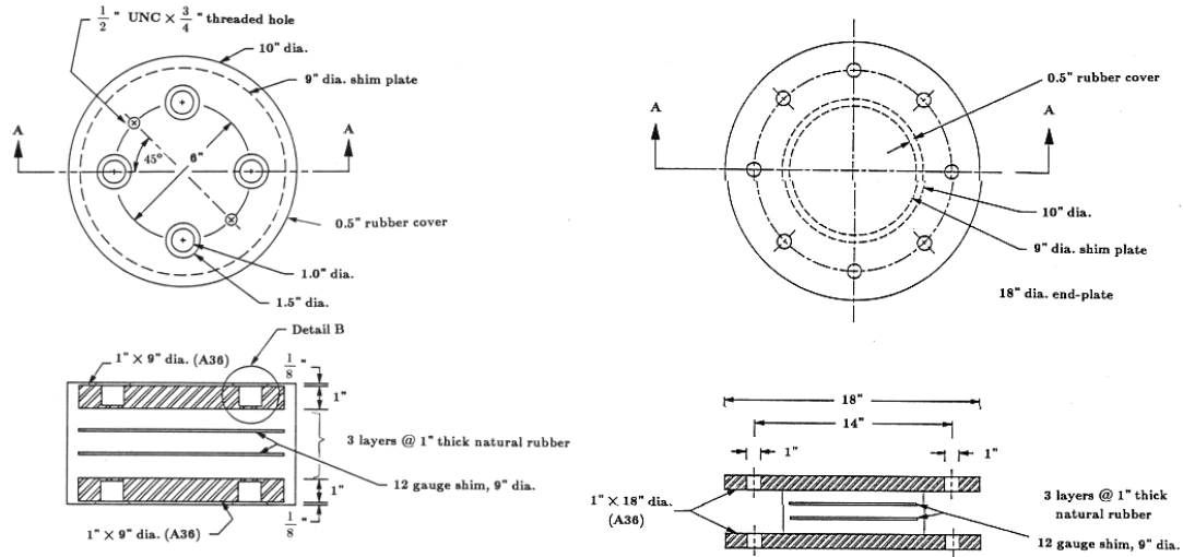
Fig. 7.2. Plan and cross section of low shape-factor rubber bearing with doweled (left) and bolted (right) end-plate connection (EERC).
