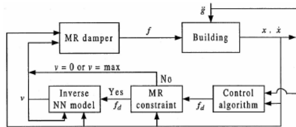
Fig. 6.1. Semiactive neural network control strategy
