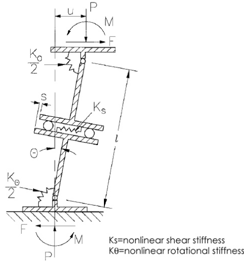
Fig. 7.21. Nonlinear analytical model developed (Nagarajaiah and Ferrell, 1999; Buckle et al., 2002)
