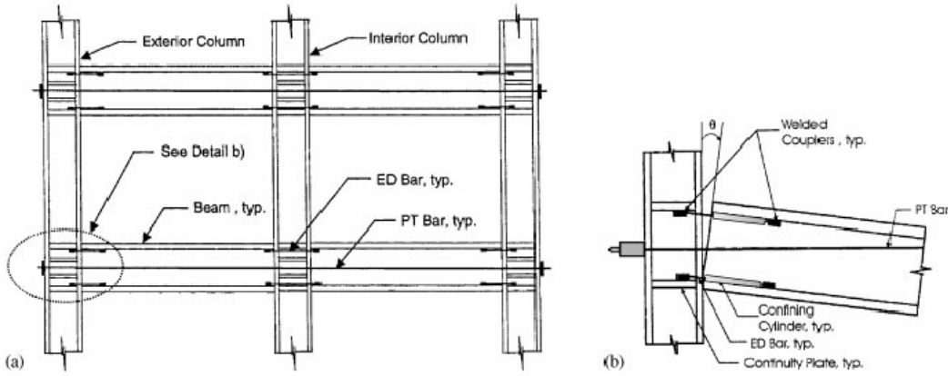
Fig. 5.16. PTED steel connection: (a) steel frame with PTED connections; (b) deformed configuration of exterior PTED connection.
