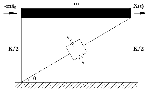
Fig. 4.18: Single storey structure equipped with viscoelastic dampers
