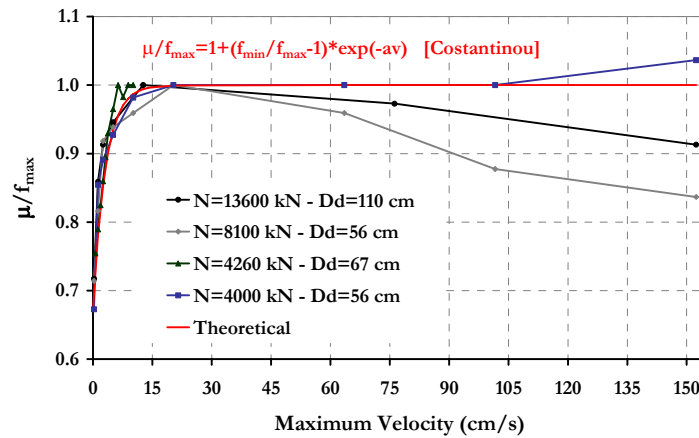
Fig. 2.13. Normalised friction coefficient-velocity dependence: theoretical vs experimental at different bearing pressures and design displacements (on the courtesy of G. Benzoni)
