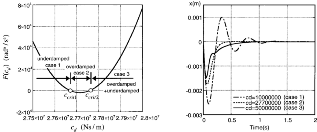
Fig. 4.20. Discriminant function of the third-order differential equation (left) and time histories of free vibration of the three analysed numerical models with different damping coefficients (right)
