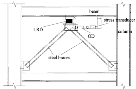
Fig. 7.22. The installation of the combined energy dissipation system in a frame
