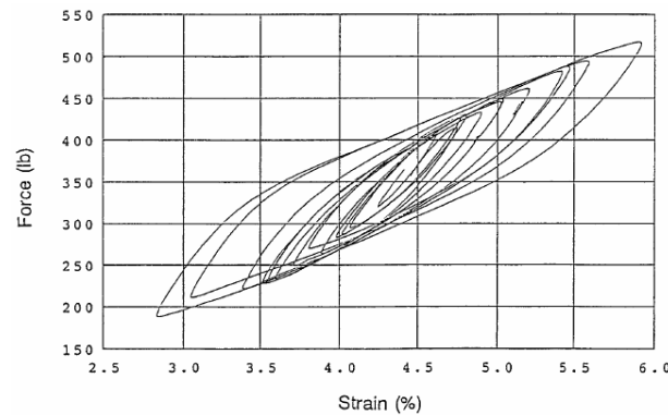
Fig. 5.7. Nitinol hysteresis behavior with pre-strain applied
