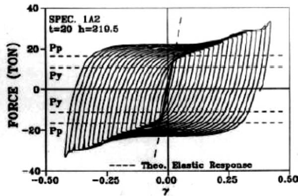
Fig. 3.20. TADAS load-deformation test results (Tsai et al.)
