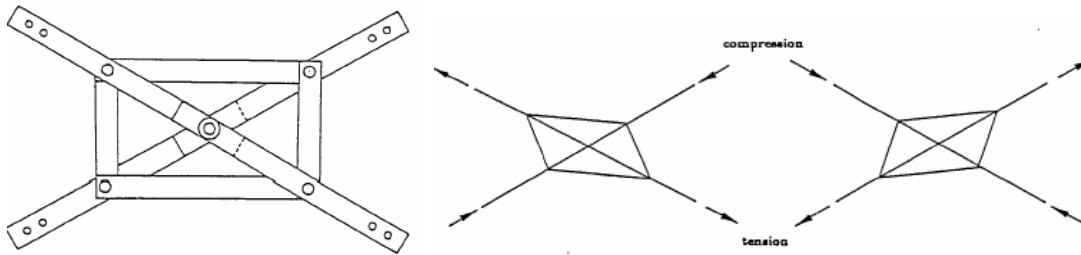
Fig. 3.6. Pall Friction Damper: Device and Deformed Configurations
