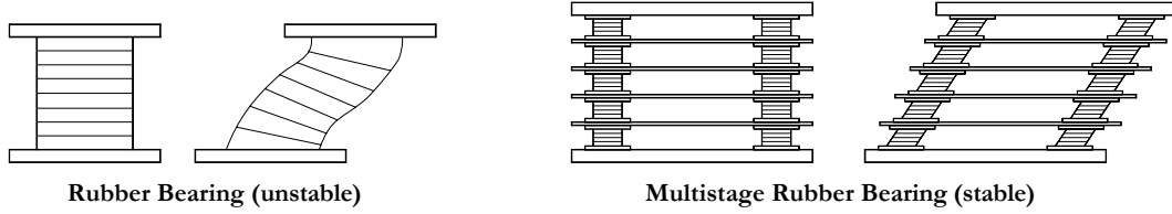
Fig. 7.10. Comparison between ordinary lamination rubber bearing and multi-stage rubber bearing
