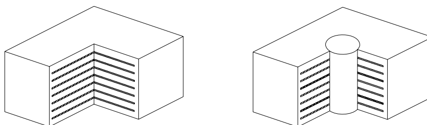
Fig. 2.20. Laminated (left) and Lead (right) Rubber Bearings
