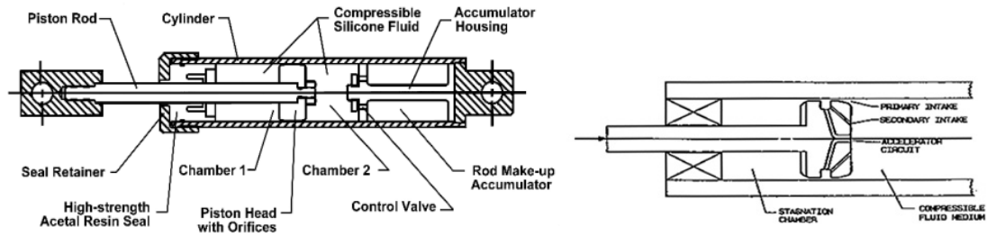
Fig. 4.5. The Taylor device (left) and detail of the fluid control orifice (right)
