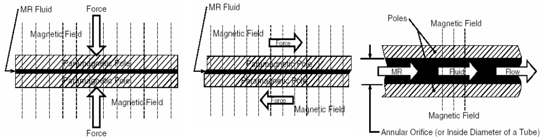
Fig. 6.2. MR fluid used in squeeze, shear and valve modes
