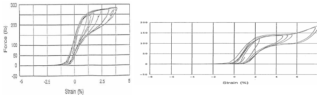
Fig. 5.6. Nitinol Moderate-Strain (up) and High-Strain (down) Hysteresis Behavior
