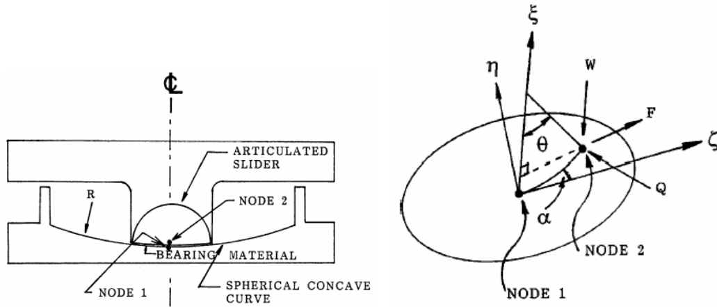
Fig. 8.10. Forces acting at nodal point 2
