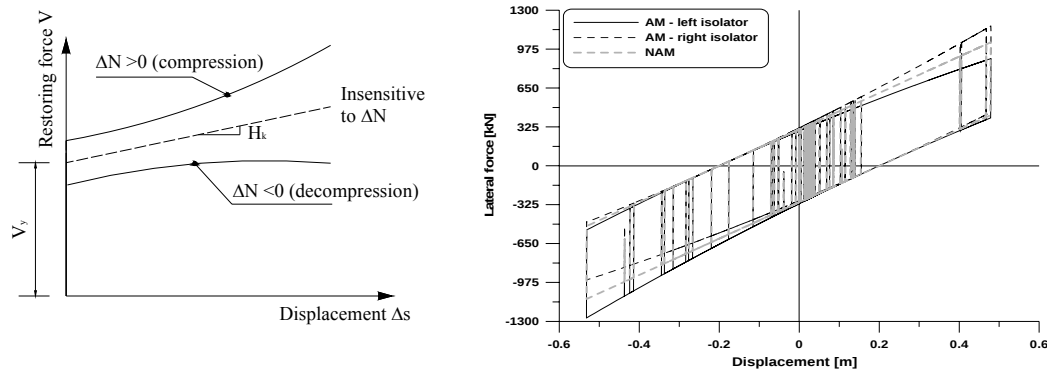
Fig. 2.23. FPS Constitutive law (left) and hysteresis loops (right): simplified and advanced models
