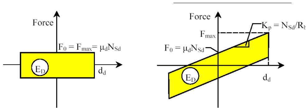
Fig. 2.19. Sliding Friction Hysteretic behaviour for Flat (left) and Curved (right) Surfaces
