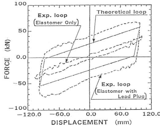
Fig. 7.8. Hysteretic loops for elastomeric bearings with and without lead plug (EERC)
