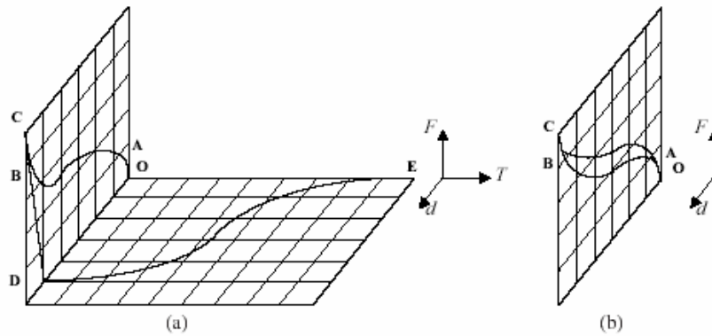
Fig. 5.4. Typical behaviour of an SMA element: shape memory effect (a) and superelasticity (b)
