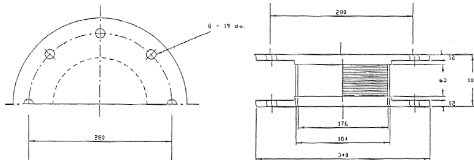
Fig. 7.5. Half plan and elevation of a typical HDRB (EERC)
