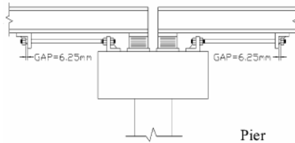
Fig. 5.2. Configuration of shape memory alloy restrainer bar used in multi-span simply supported bridges
