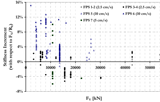
Fig. 8.7. Test results on FPS, variation of the stiffness device with the bearing pressure
