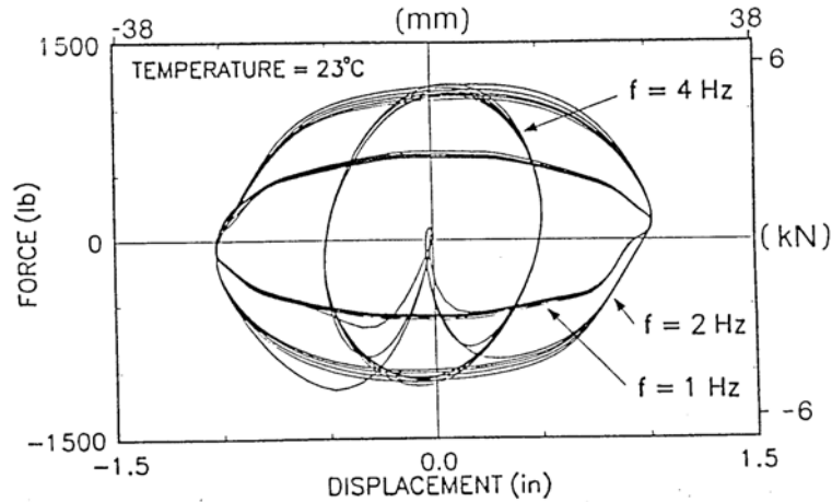
Fig. 4.6. Experimental hysteresis loop of a Taylor fluid damper at various frequencies and temperatures (Constantinou et al. 1993)
