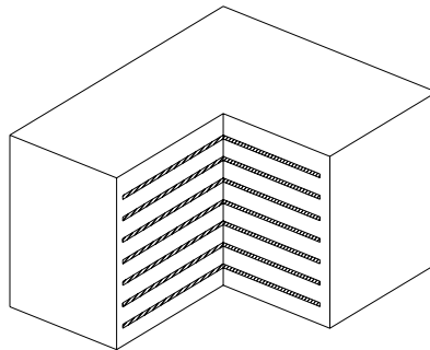
Fig. 7.1. Schematic design of a laminated natural rubber bearing
